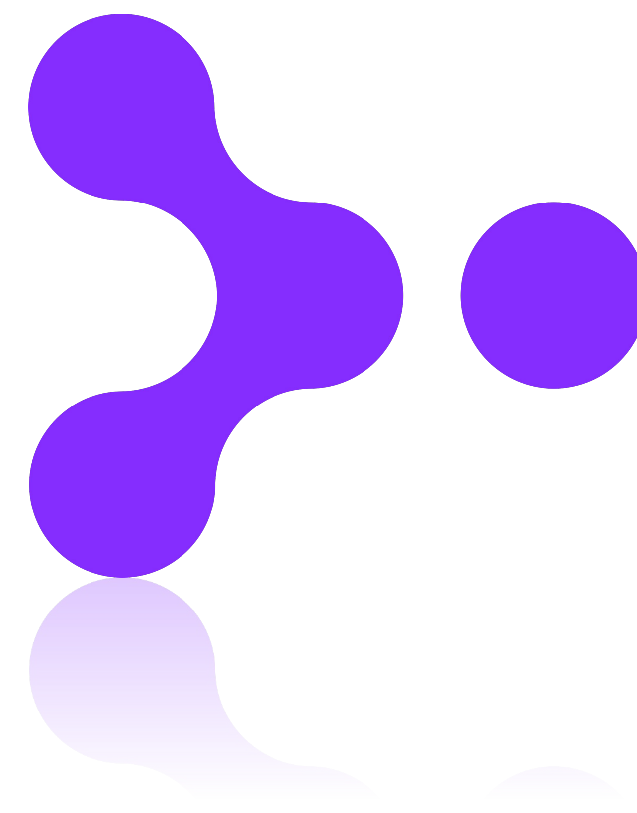
Mesh Network
