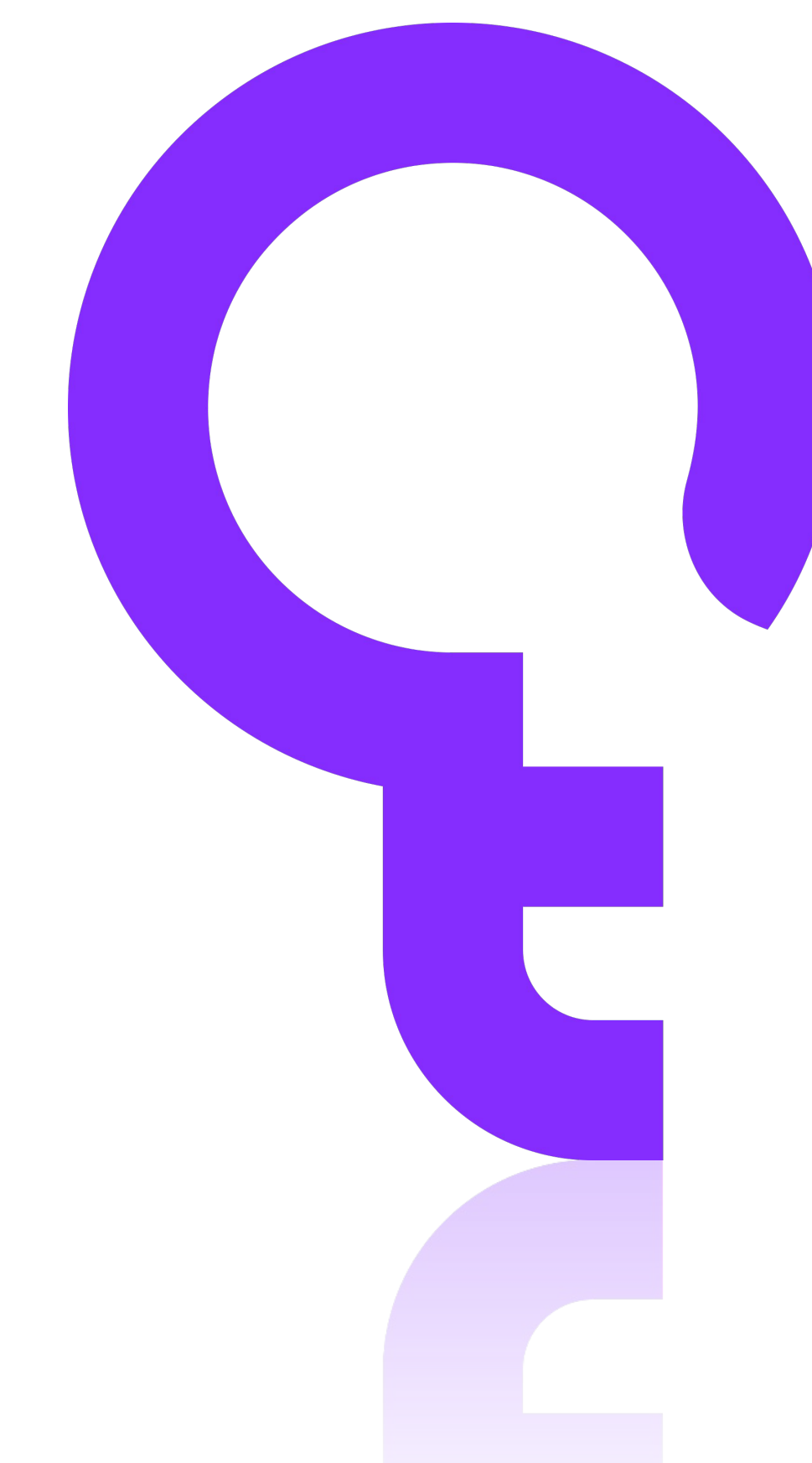
Password Manager
